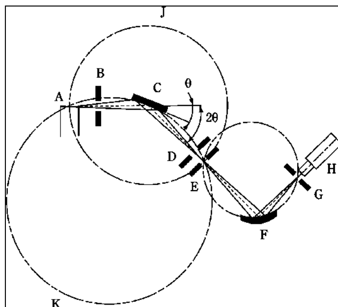
Figure 3 – Geometrical arrangement of the Bragg-Brentano para-focal geometry.
