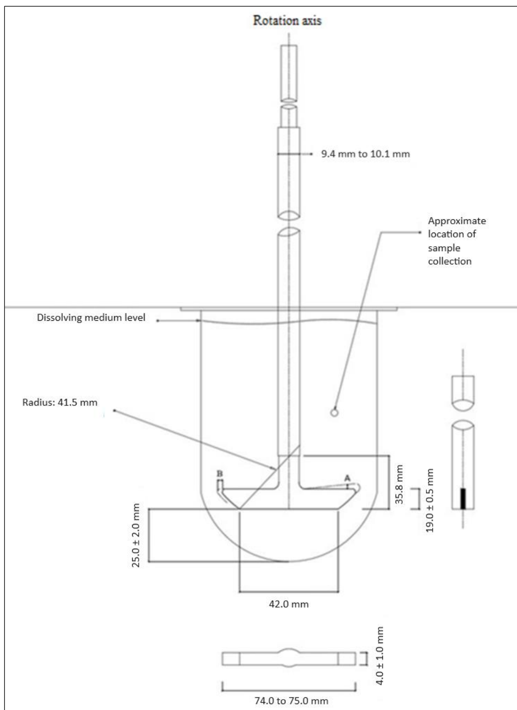
Figure 2 - Method 2 (Paddles). The paddle and the tank are not in the same size promotion.
