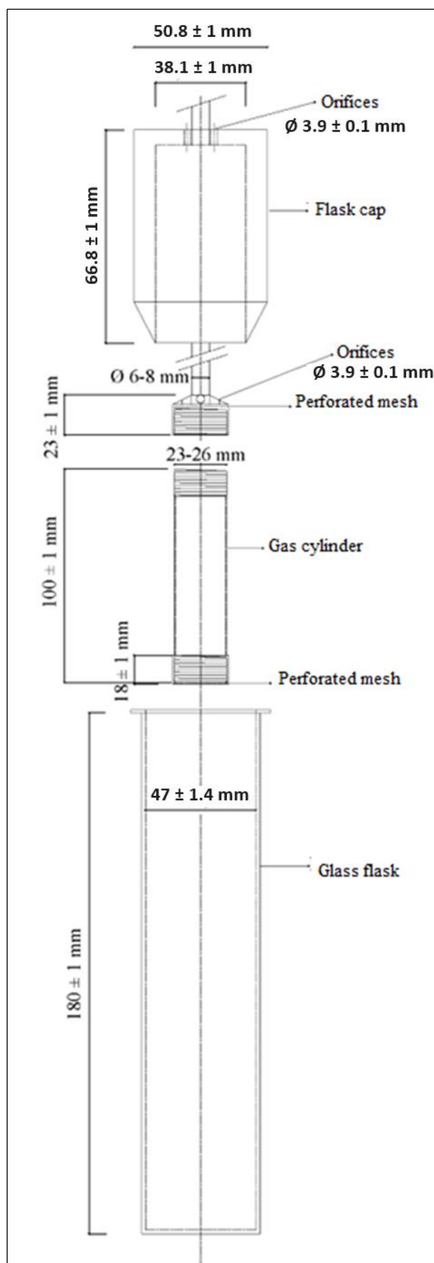
Figure 3 – Method 3 (Alternate Cylinders). The symbol \varnothing corresponds to the diameter
