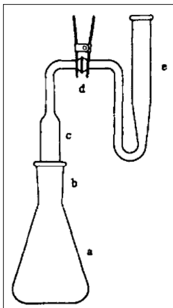
Figure 1 – Arsenic determination system using the spectrophotometric method.
