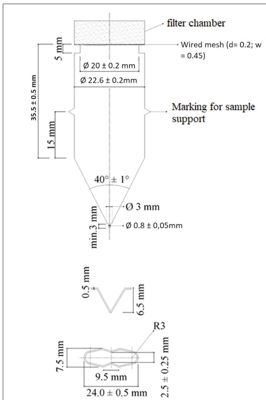
Figure 4 - Method 4 (Flow-cell). Large cell for tablets and capsules (upper part); tablet holder for the large cell (lower part). The symbol \varnothing corresponds to diameter.
