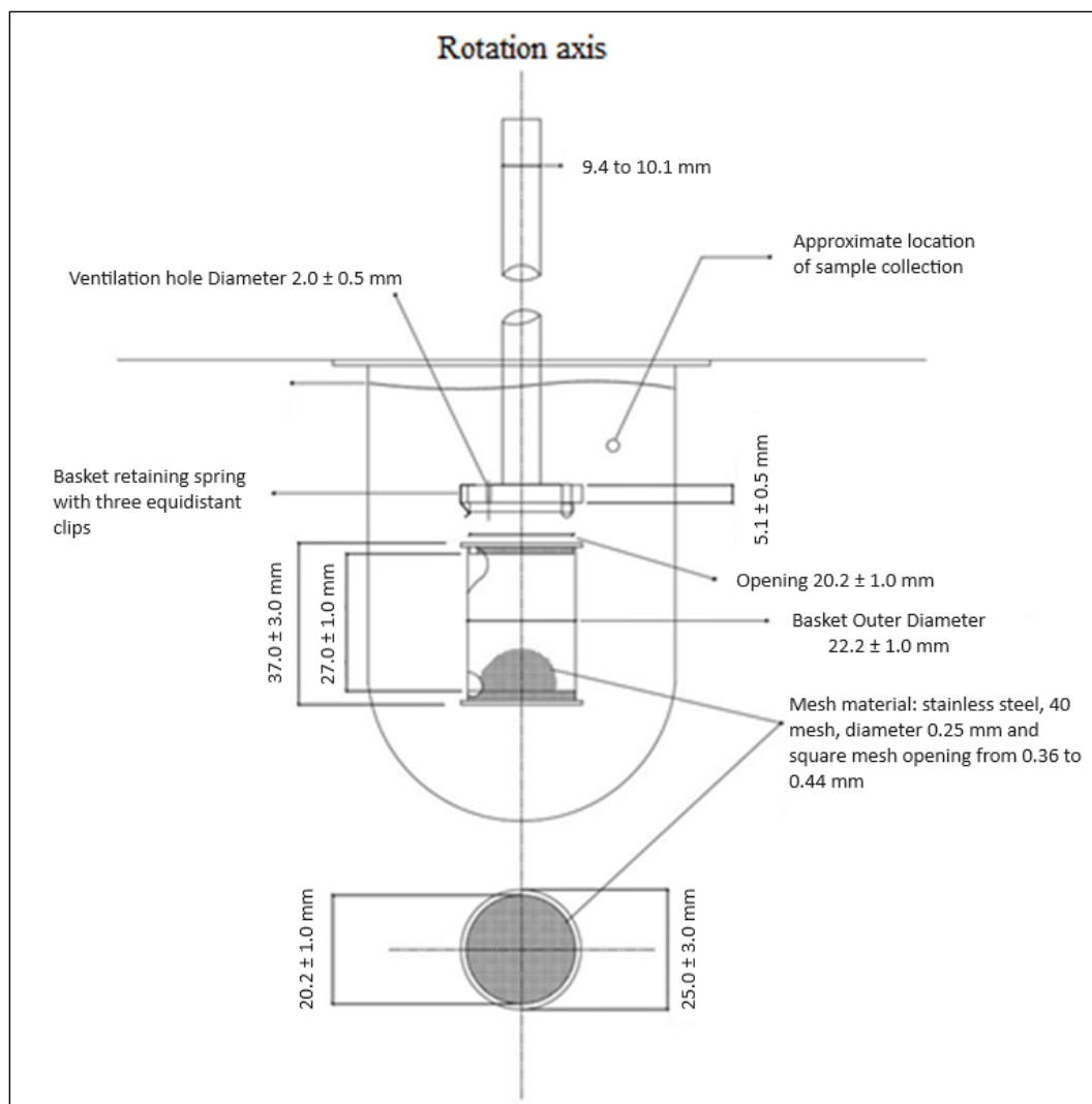
Figure 1 - Method 1 (Baskets). The basket and the tank are not in the same size proportion.
