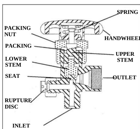
Figure 2 – Cylinder valve.
