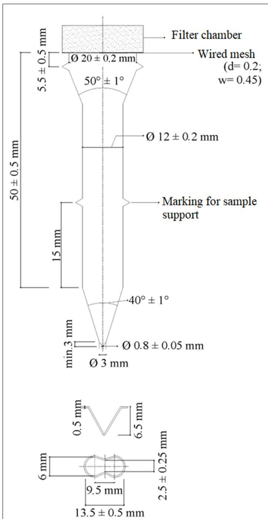
Figure 5 - Method 4 (Flow-cell). Small cell for tablets and capsules (upper part); tablet holder for the small cell (lower part). The symbol Ø corresponds to diameter
